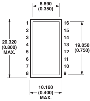
HLCP-H100 HLMP-2x85
