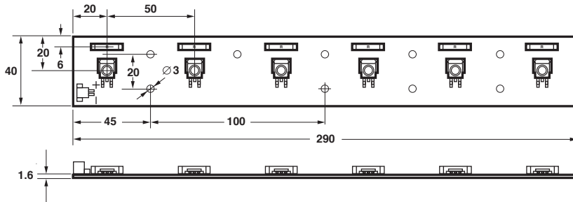
ADJD-xM21 (6 LEDs)
