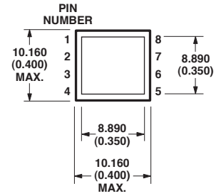
HLCP-C100 HLMP-2x55
